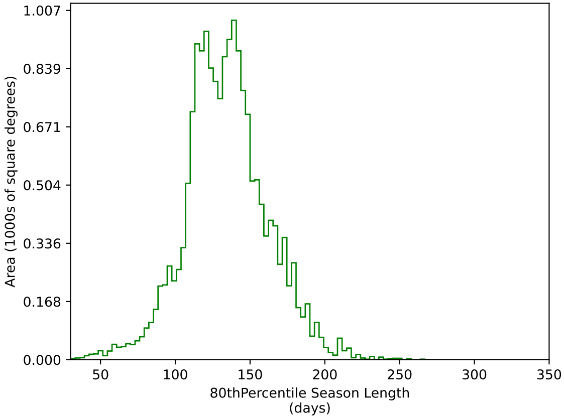
too_elab_heavy_r128_d3_gz_v3.4_10yrs WFD g band: 80thPercentile Season Length
