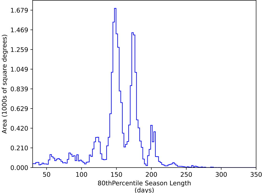
too_elab_heavy_r128_d3_gz_v3.4_10yrs All sky y band: 80thPercentile Season Length
