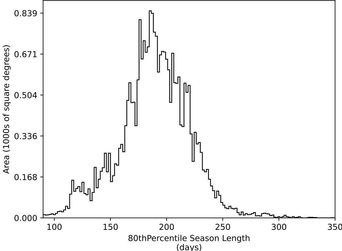
too_elab_heavy_r128_d3_gz_v3.4_10yrs All sky all bands: 80thPercentile Season Length
