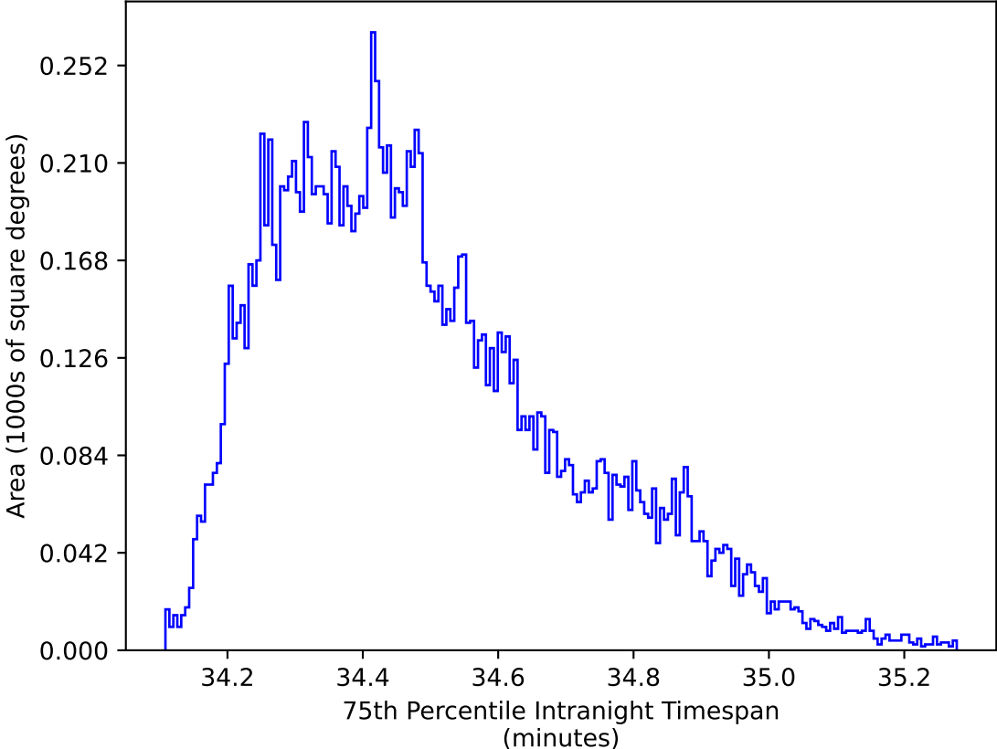
too_elab_heavy_r128_d3_gz_v3.4_10yrs WFD zy bands: 75th Percentile Intranight Timespan
