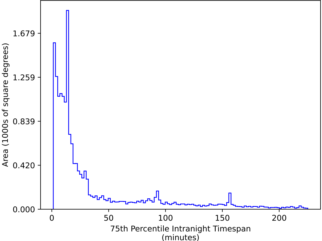
too_elab_heavy_r128_d3_gz_v3.4_10yrs WFD z band: 75th Percentile Intranight Timespan
