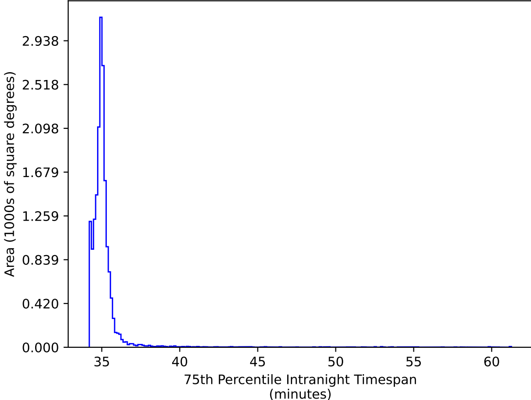
too_elab_heavy_r128_d3_gz_v3.4_10yrs WFD ri bands: 75th Percentile Intranight Timespan
