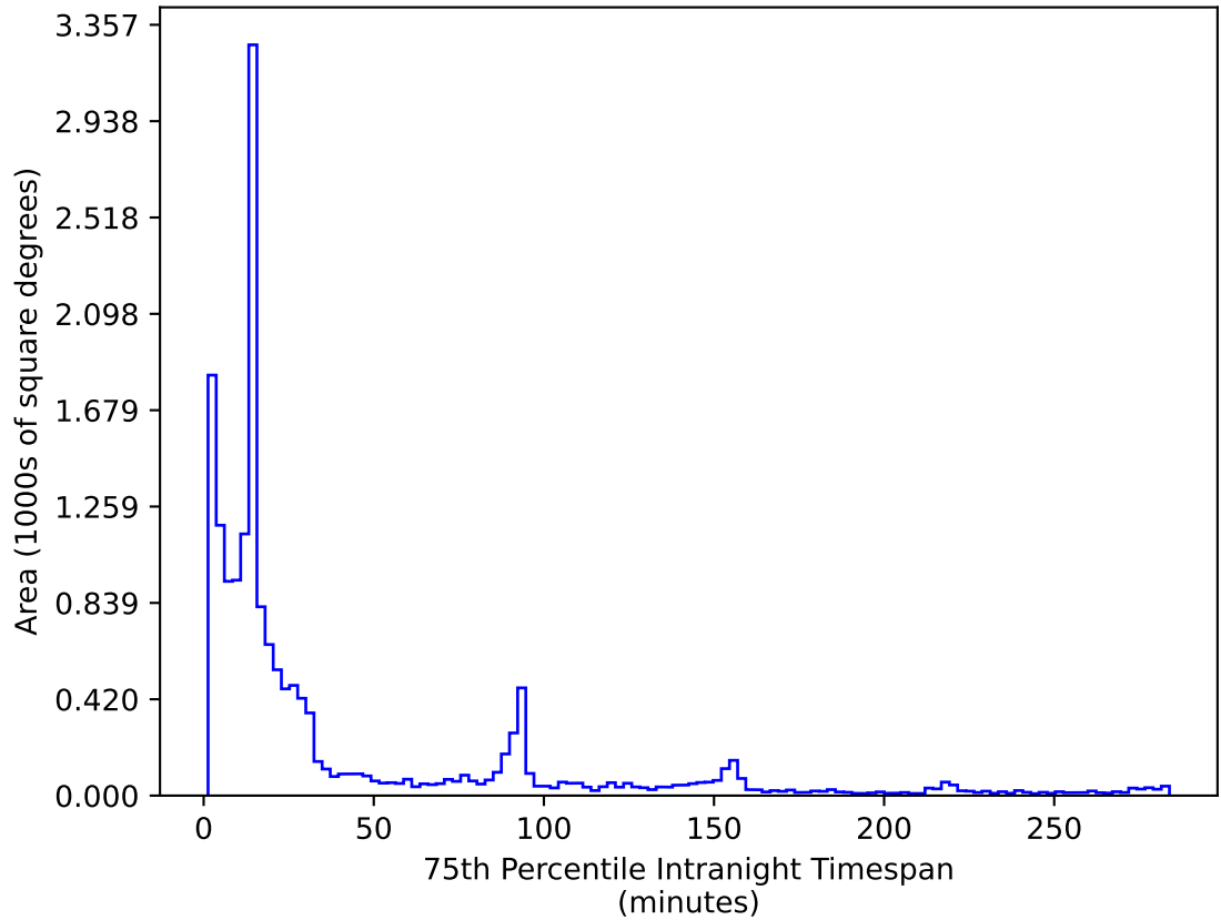
too_elab_heavy_r128_d3_gz_v3.4_10yrs WFD r band: 75th Percentile Intranight Timespan
