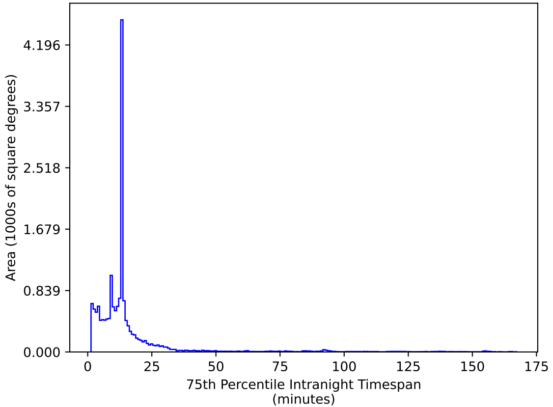
too_elab_heavy_r128_d3_gz_v3.4_10yrs WFD i band: 75th Percentile Intranight Timespan
