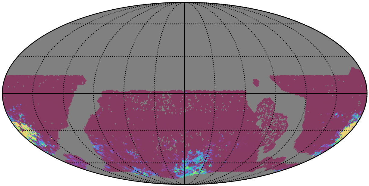
too_elab_heavy_r128_d3_gz_v3.4_10yrs WFD gr bands: 75th Percentile Intranight Timespan
