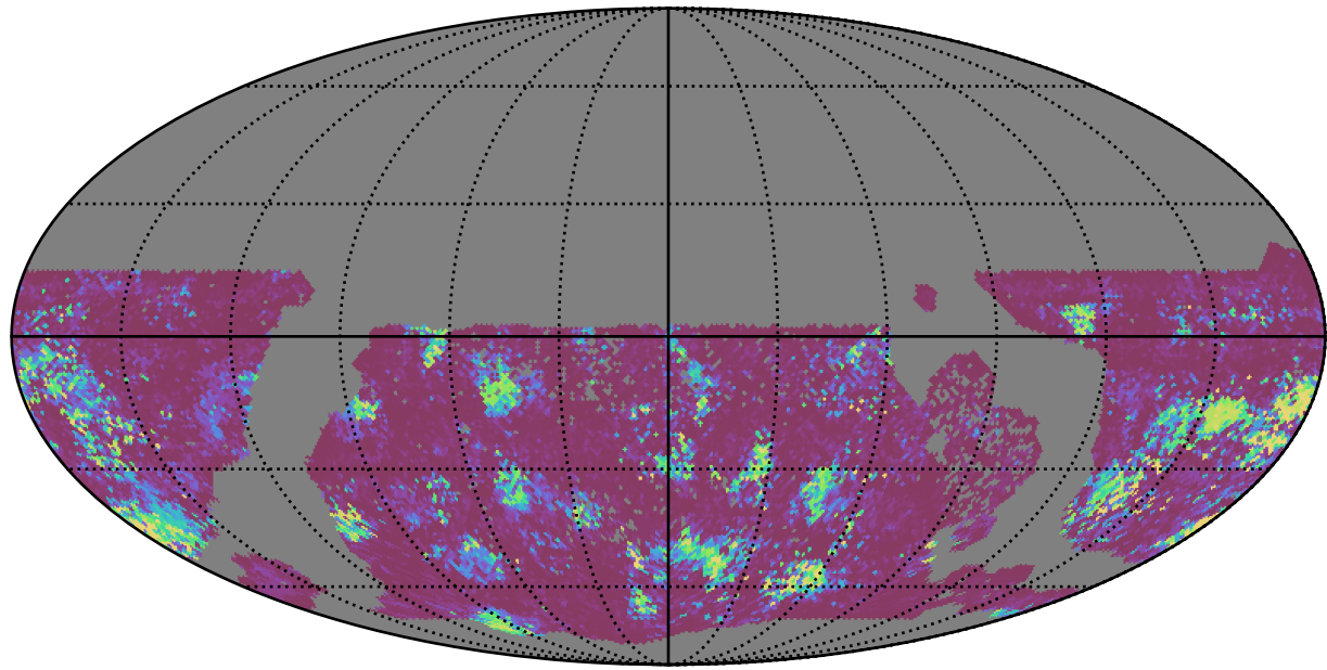
too_elab_heavy_r128_d3_gz_v3.4_10yrs WFD g band: 75th Percentile Intranight Timespan
