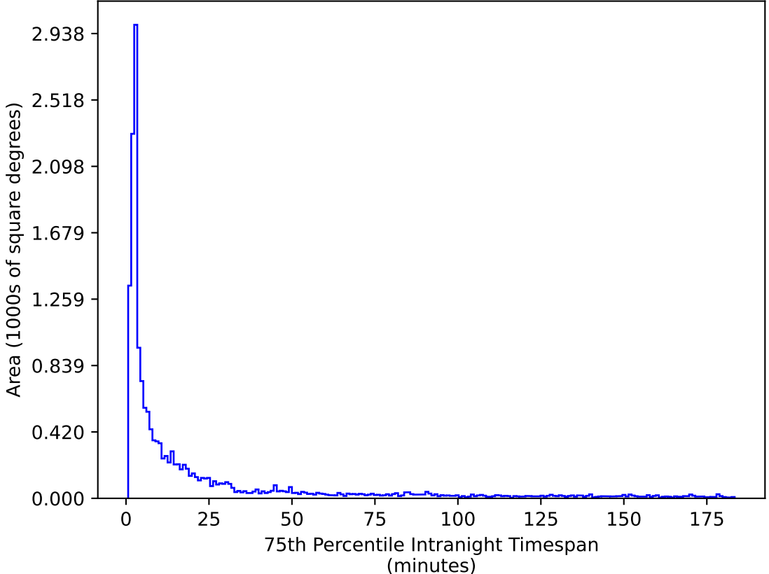
too_elab_heavy_r128_d3_gz_v3.4_10yrs WFD g band: 75th Percentile Intranight Timespan
