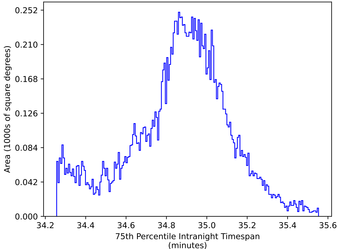
too_elab_heavy_r128_d3_gz_v3.4_10yrs WFD: 75th Percentile Intranight Timespan
