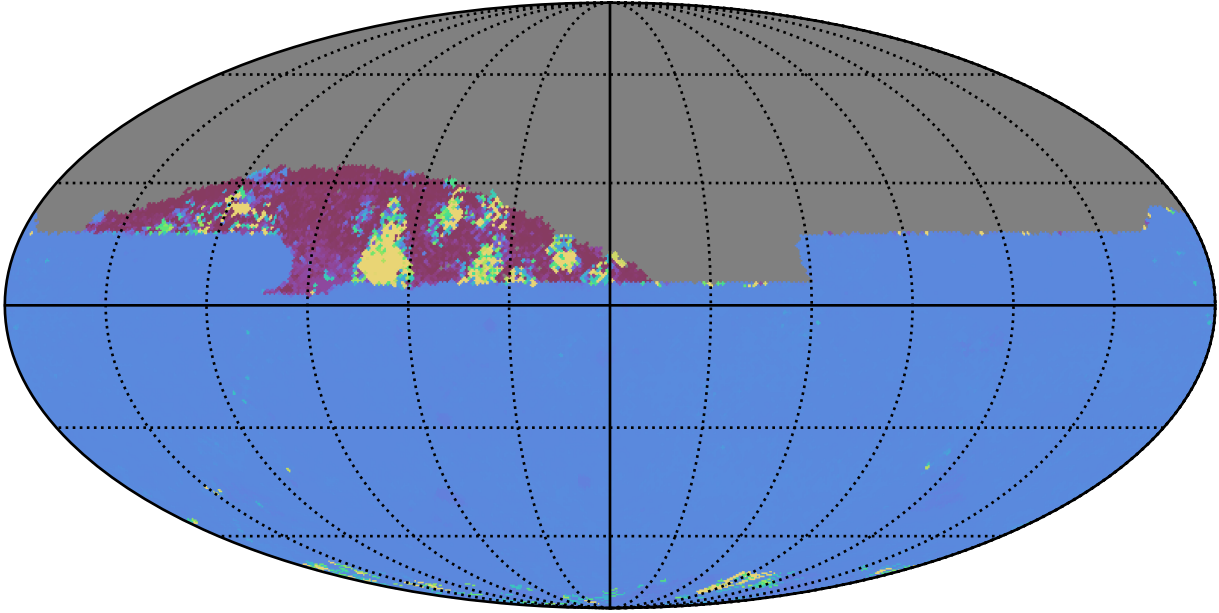
too_elab_heavy_r128_d3_gz_v3.4_10yrs All sky zy bands: 75th Percentile Intranight Timespan
