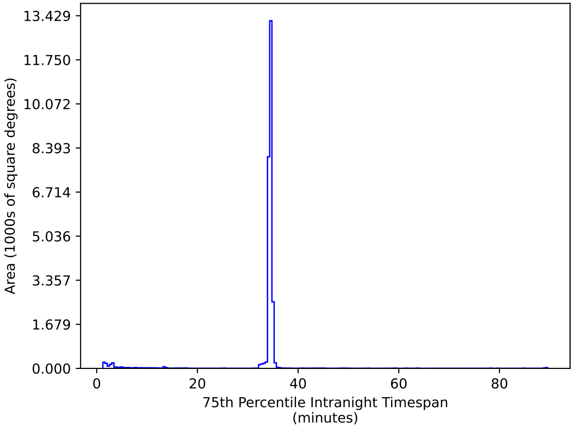
too_elab_heavy_r128_d3_gz_v3.4_10yrs All sky zy bands: 75th Percentile Intranight Timespan
