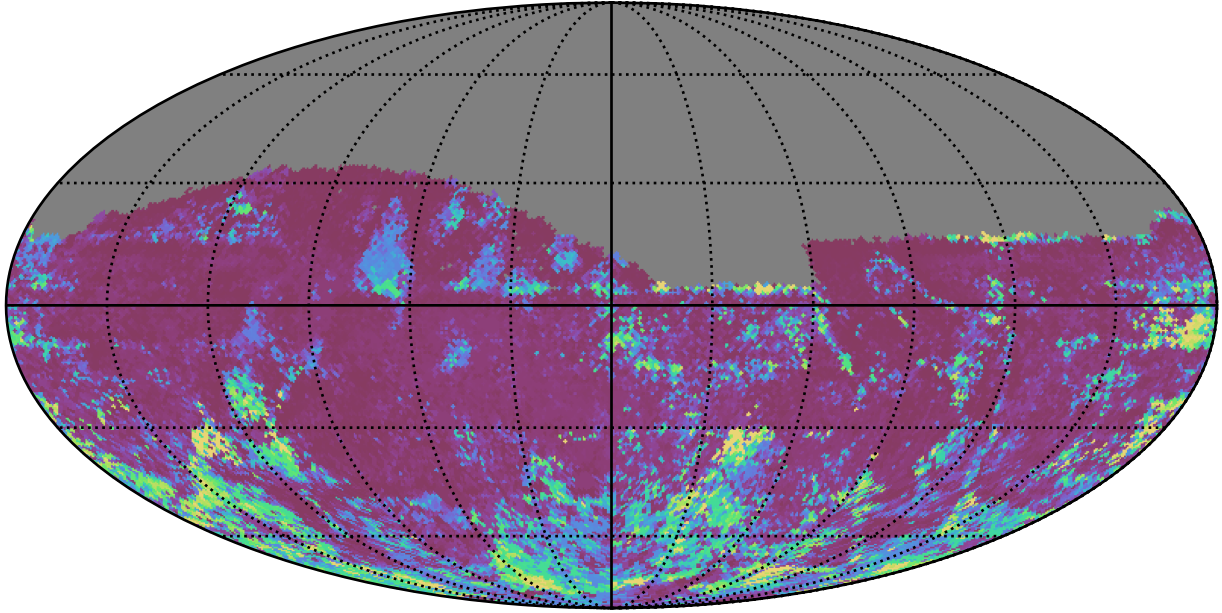
too_elab_heavy_r128_d3_gz_v3.4_10yrs All sky z band: 75th Percentile Intranight Timespan
