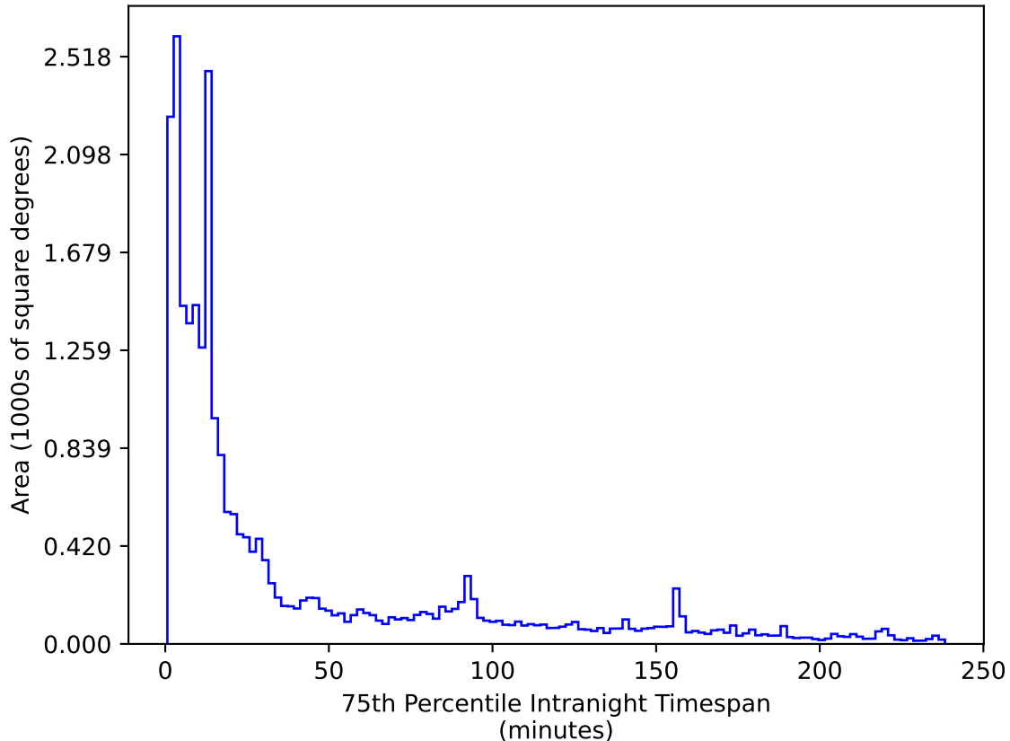
too_elab_heavy_r128_d3_gz_v3.4_10yrs All sky z band: 75th Percentile Intranight Timespan
