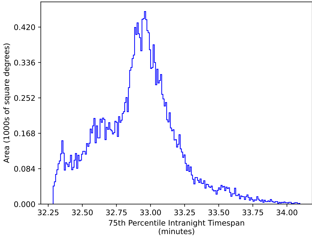
too_elab_heavy_r128_d3_gz_v3.4_10yrs All sky y band: 75th Percentile Intranight Timespan
