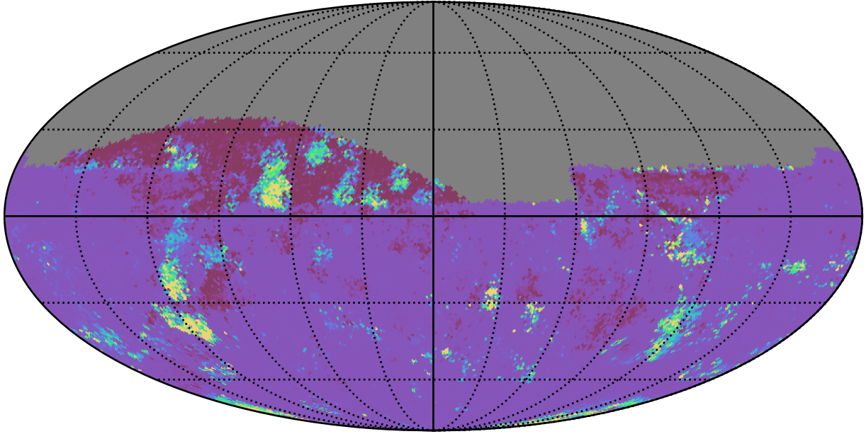
too_elab_heavy_r128_d3_gz_v3.4_10yrs All sky ug bands: 75th Percentile Intranight Timespan
