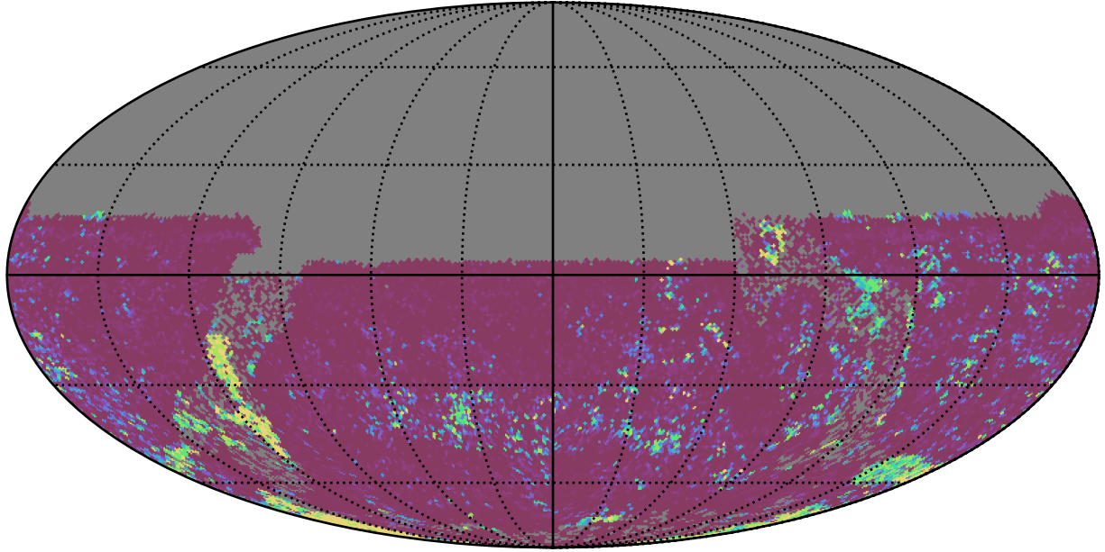
too_elab_heavy_r128_d3_gz_v3.4_10yrs All sky u band: 75th Percentile Intranight Timespan
