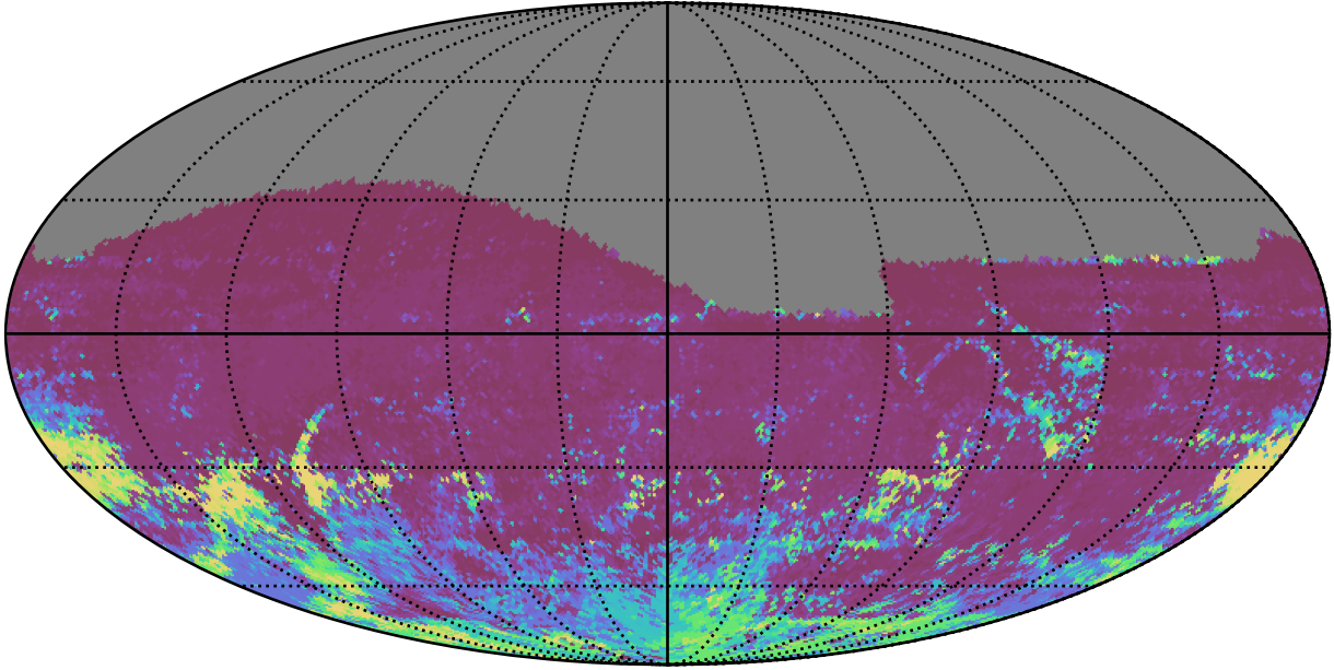
too_elab_heavy_r128_d3_gz_v3.4_10yrs All sky r band: 75th Percentile Intranight Timespan
