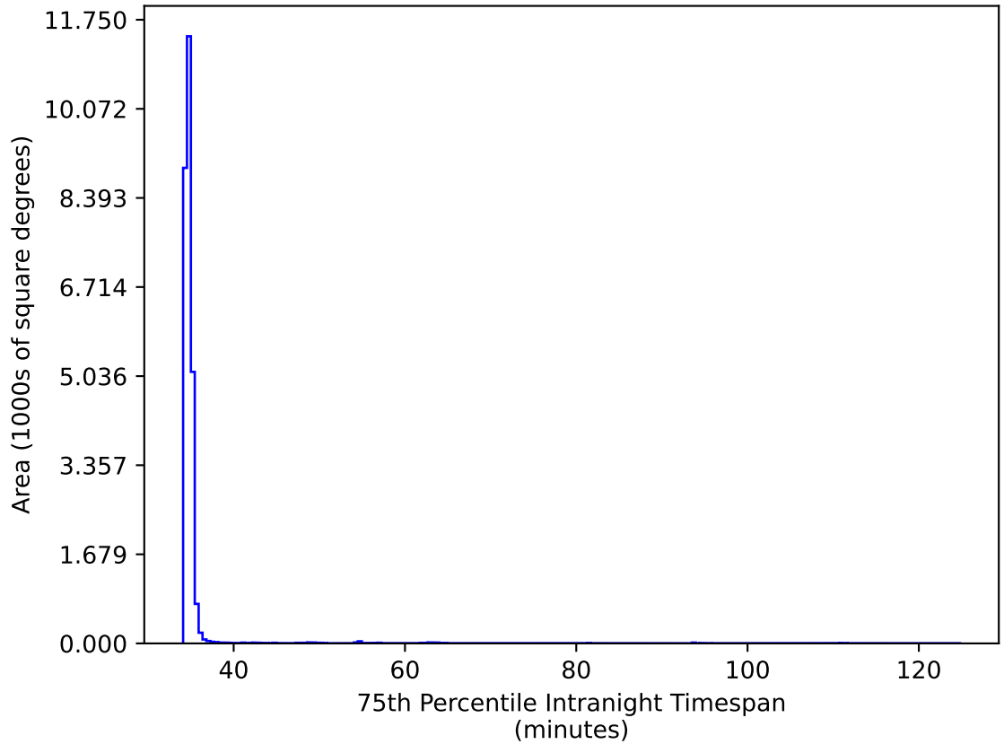
too_elab_heavy_r128_d3_gz_v3.4_10yrs All sky iz bands: 75th Percentile Intranight Timespan
