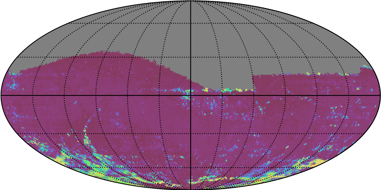
too_elab_heavy_r128_d3_gz_v3.4_10yrs All sky i band: 75th Percentile Intranight Timespan
