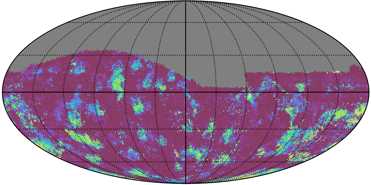
too_elab_heavy_r128_d3_gz_v3.4_10yrs All sky g band: 75th Percentile Intranight Timespan
