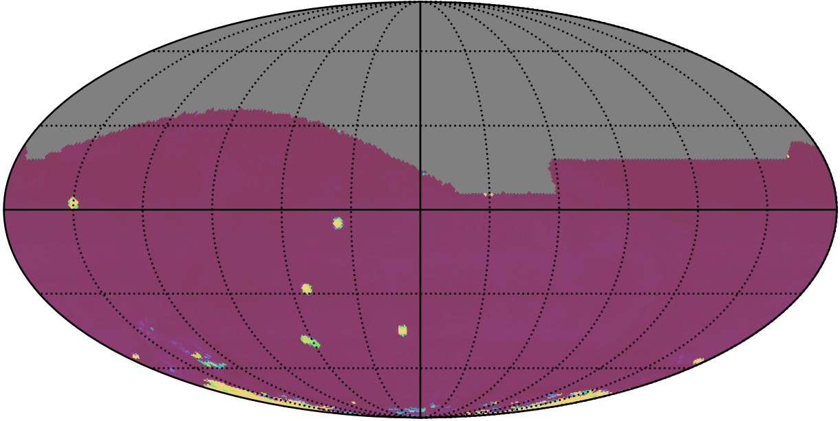
too_elab_heavy_r128_d3_gz_v3.4_10yrs All sky all bands: 75th Percentile Intranight Timespan
