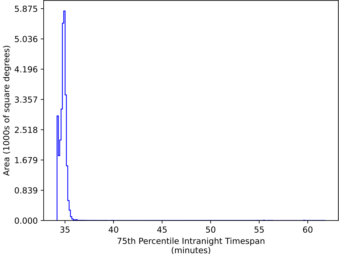
too_elab_heavy_r128_d3_gz_v3.4_10yrs All sky: 75th Percentile Intranight Timespan
