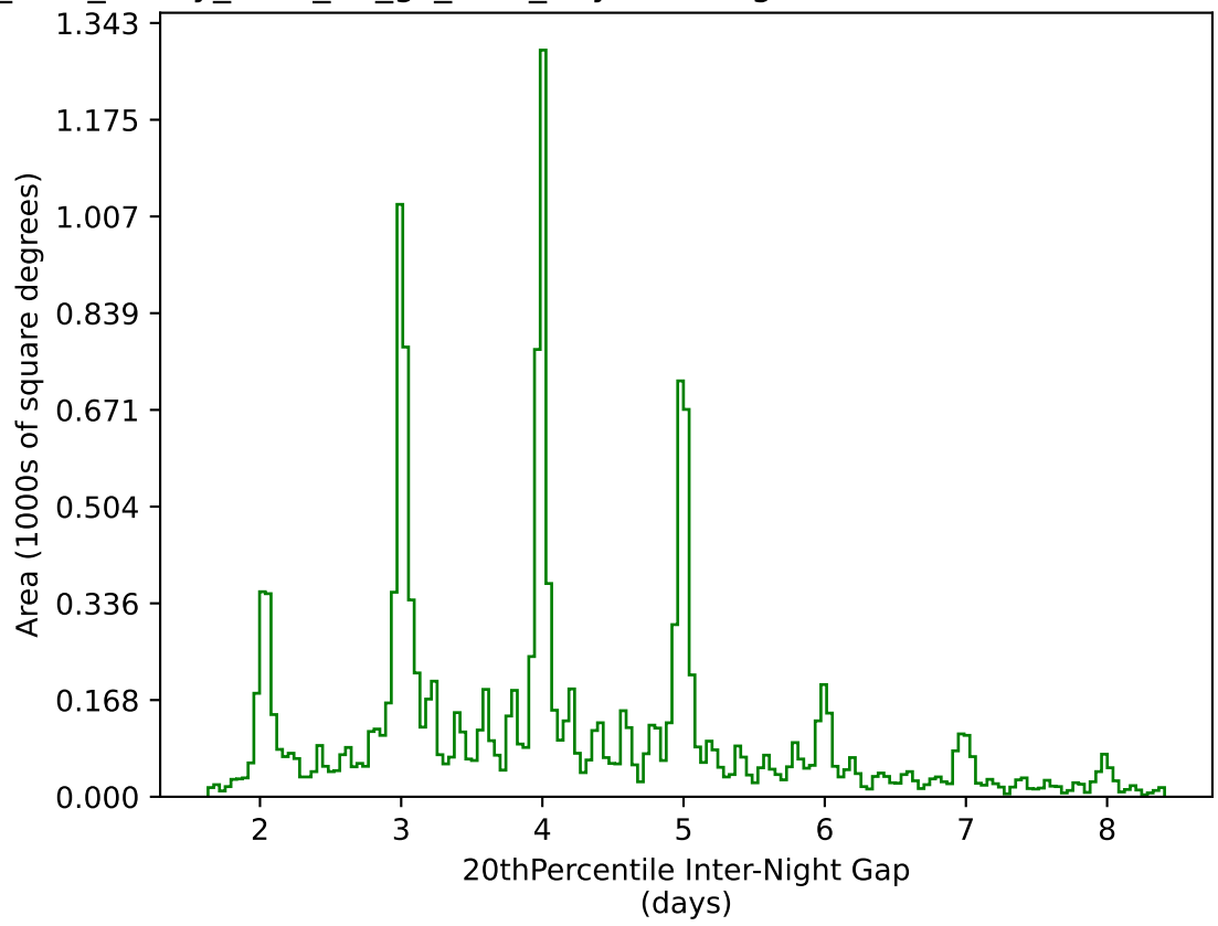
too_elab_heavy_r128_d3_gz_v3.4_10yrs WFD g band: 20thPercentile Inter-Night Gap
