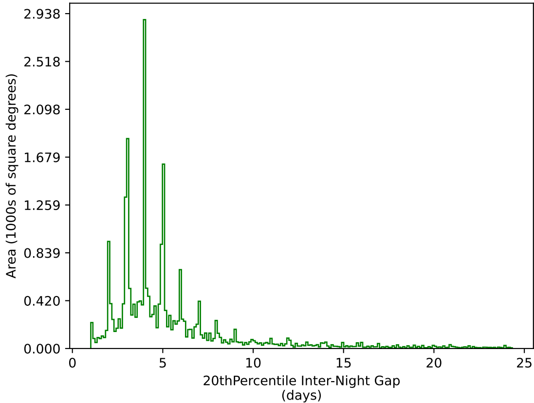
too_elab_heavy_r128_d3_gz_v3.4_10yrs All sky g band: 20thPercentile Inter-Night Gap
