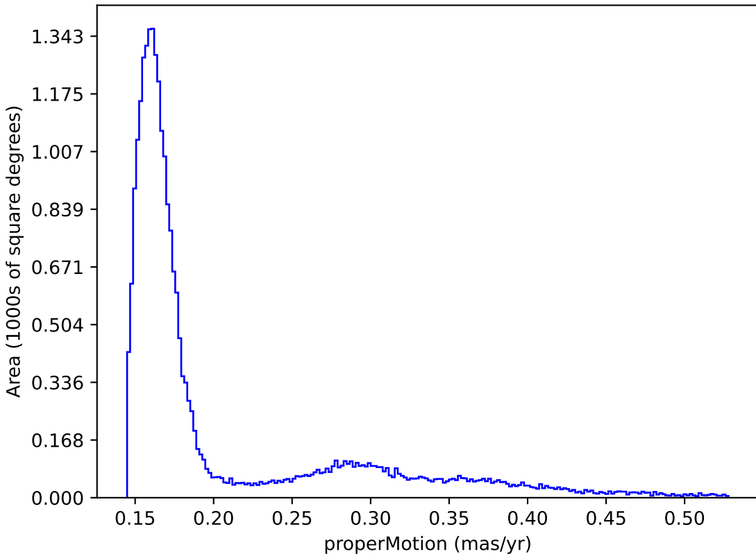
too_elab_heavy_r128_d3_gz_v3.4_10yrs : properMotion
