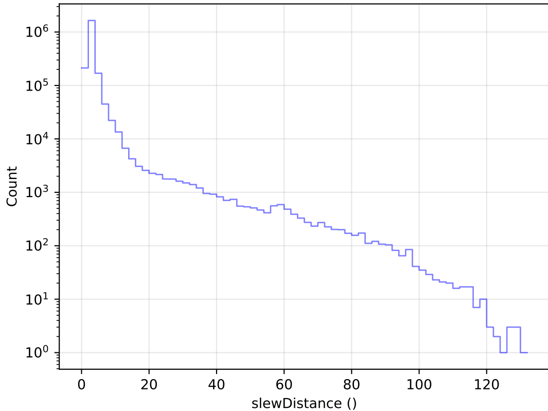
too_elab_heavy_r128_d3_gz_v3.4_10yrs All visits: Slew Distance Histogram
