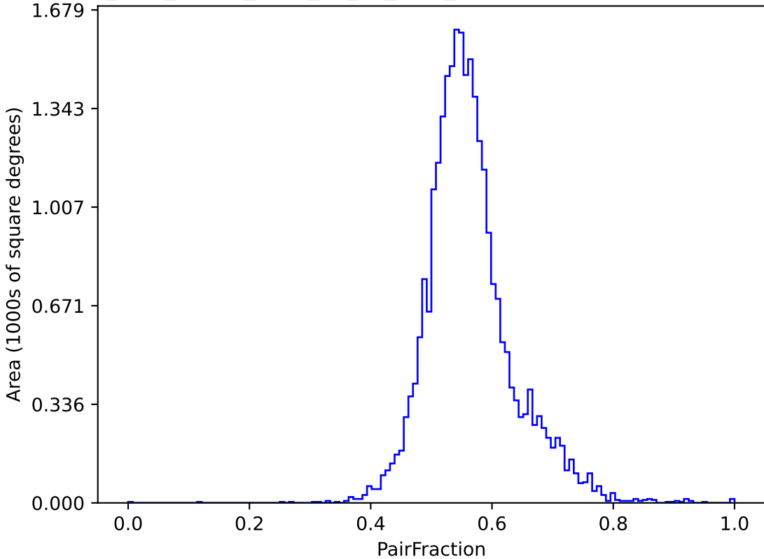
too_elab_heavy_r128_d3_gz_v3.4_10yrs (g or r or i): PairFraction
