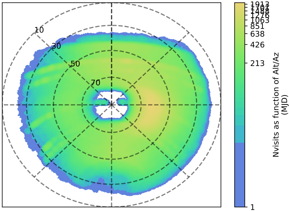
too_elab_heavy_r128_d3_gz_v3.4_10yrs y: Nvisits as function of Alt/Az
