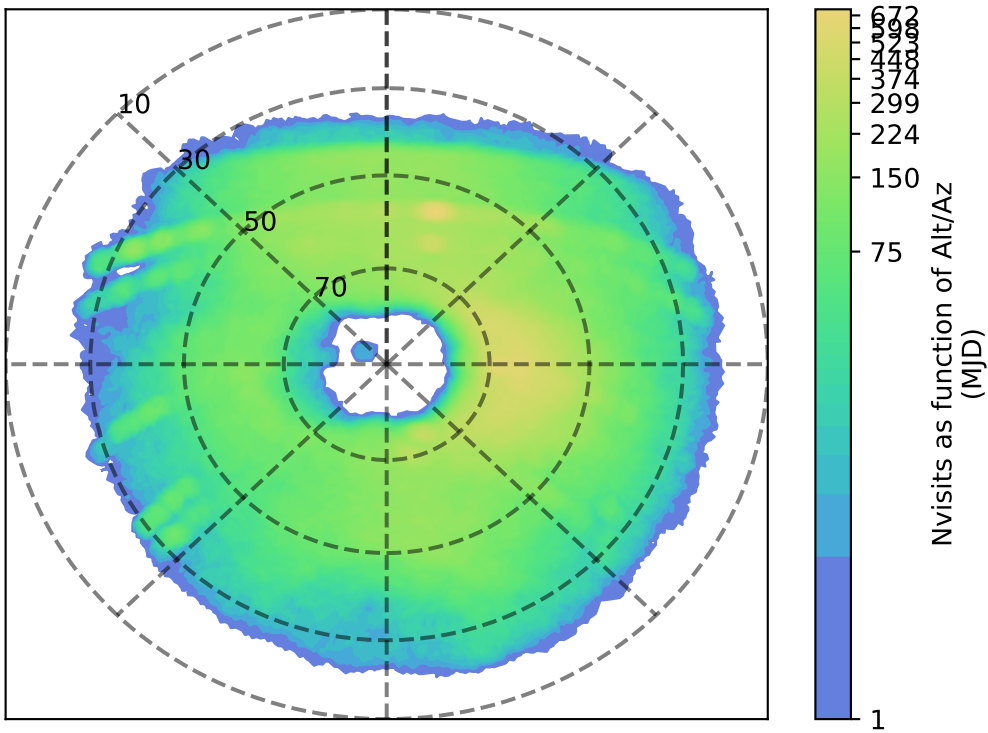
too_elab_heavy_r128_d3_gz_v3.4_10yrs u: Nvisits as function of Alt/Az
