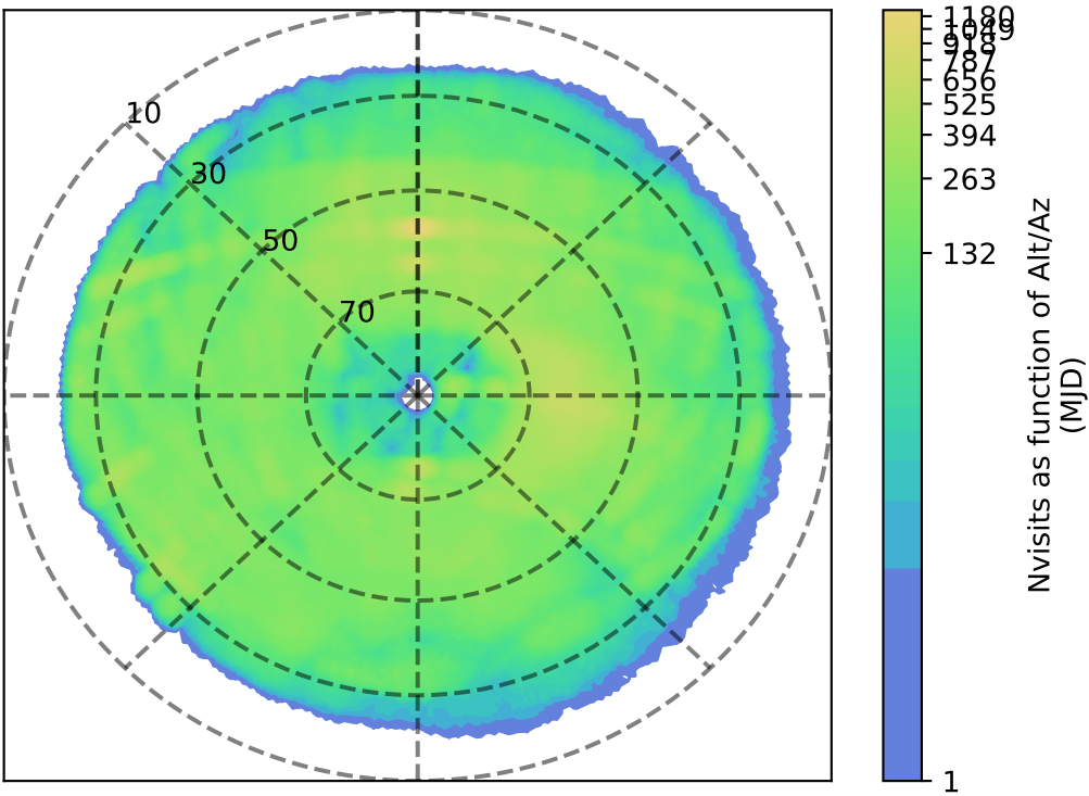
too_elab_heavy_r128_d3_gz_v3.4_10yrs g: Nvisits as function of Alt/Az
