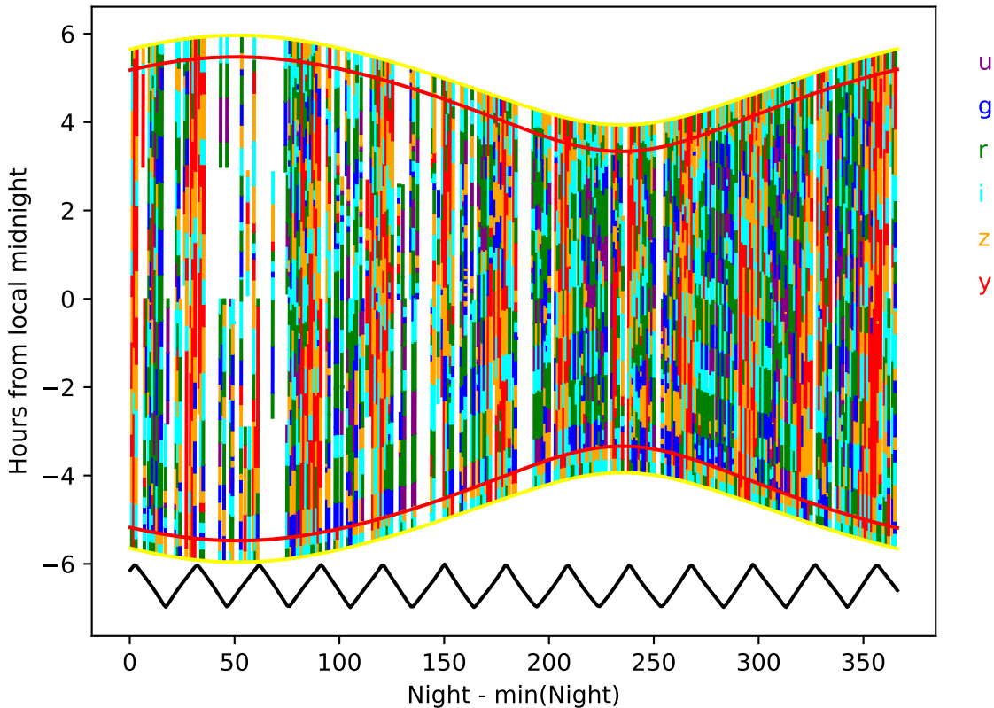
too_elab_heavy_r128_d3_gz_v3.4_10yrs year 9-10: Hourglass
