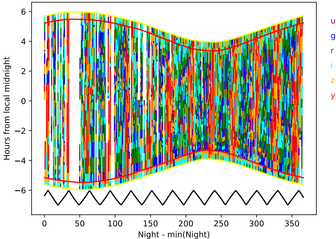
too_elab_heavy_r128_d3_gz_v3.4_10yrs year 6-7: Hourglass
