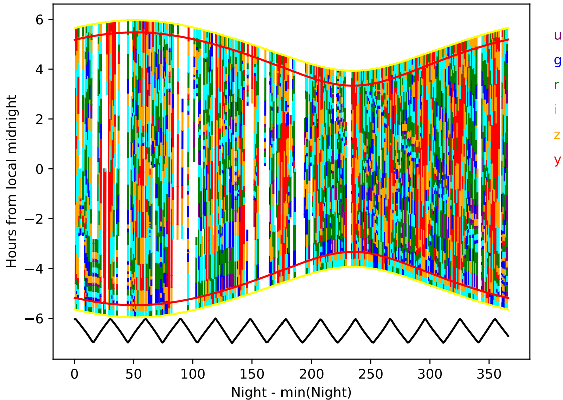
too_elab_heavy_r128_d3_gz_v3.4_10yrs year 1-2: Hourglass
