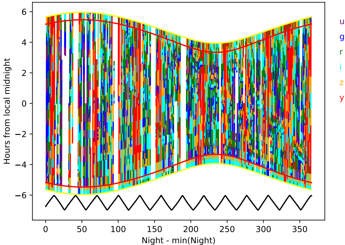
too_elab_heavy_r128_d3_gz_v3.4_10yrs year 0-1: Hourglass
