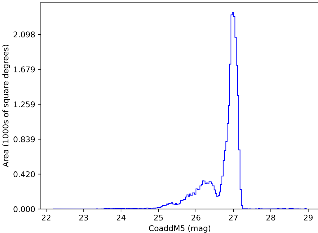
too_elab_heavy_r128_d3_gz_v3.4_10yrs r: CoaddM5
