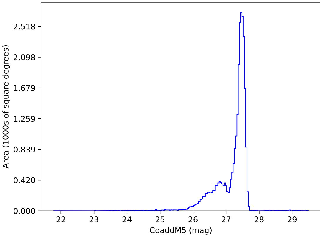
too_elab_heavy_r128_d3_gz_v3.4_10yrs : CoaddM5
