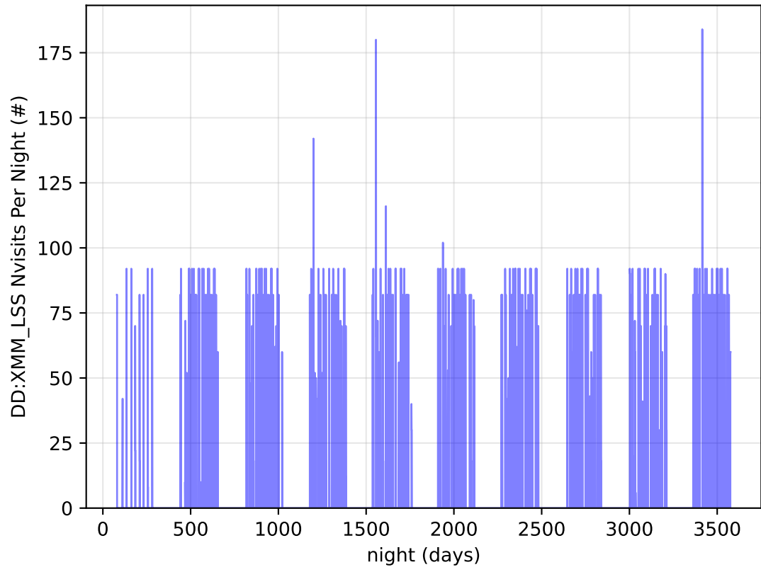
too_elab_heavy_r128_d3_gz_v3.4_10yrs all bands: DD:XMM_LSS Nvisits Per Night
