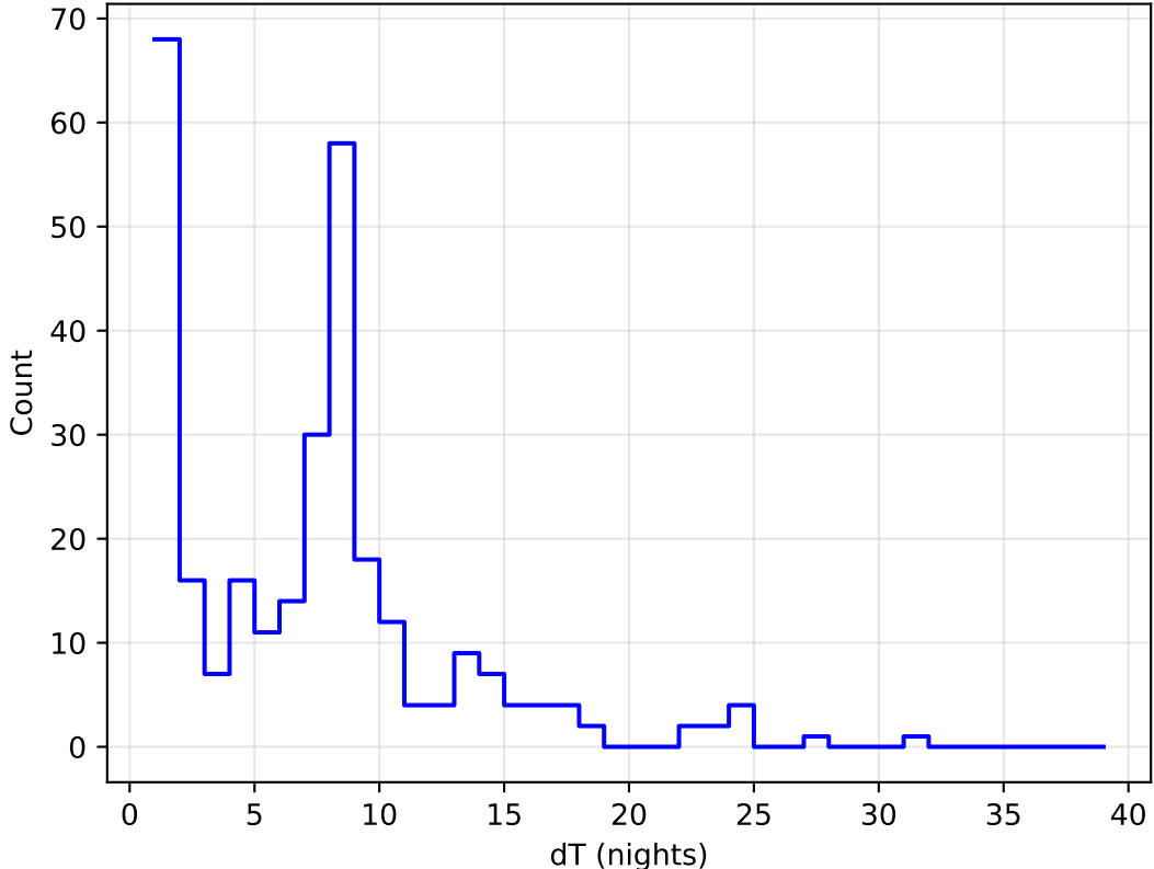
too_elab_heavy_r128_d3_gz_v3.4_10yrs all bands: DD:XMM_LSS Delta Nights Histogram
