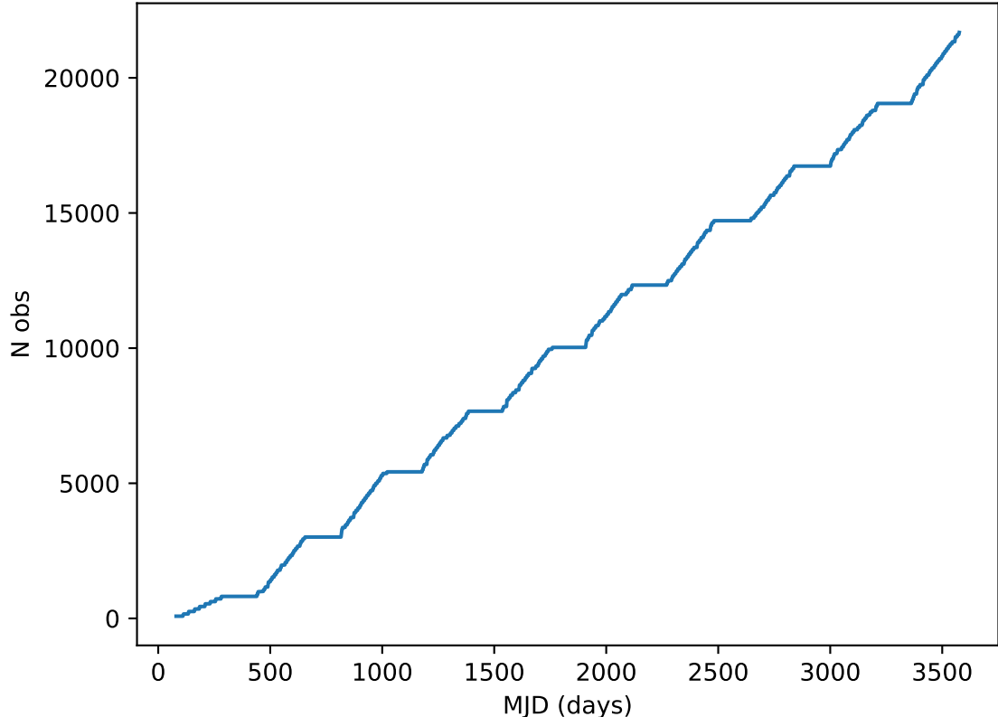
too_elab_heavy_r128_d3_gz_v3.4_10yrs all bands: DD:XMM_LSS Cumulative NVisits
