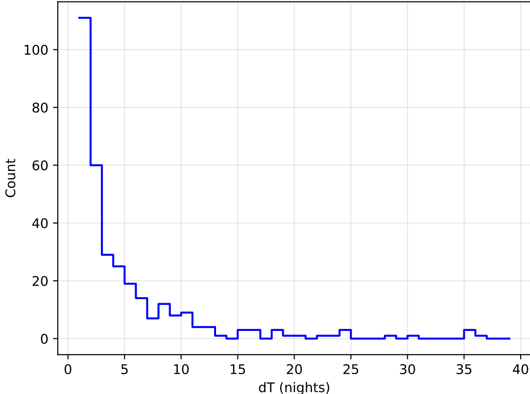
too_elab_heavy_r128_d3_gz_v3.4_10yrs all bands: DD:WFD Delta Nights Histogram
