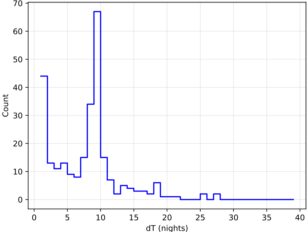
too_elab_heavy_r128_d3_gz_v3.4_10yrs all bands: DD:ELAISS1 Delta Nights Histogram
