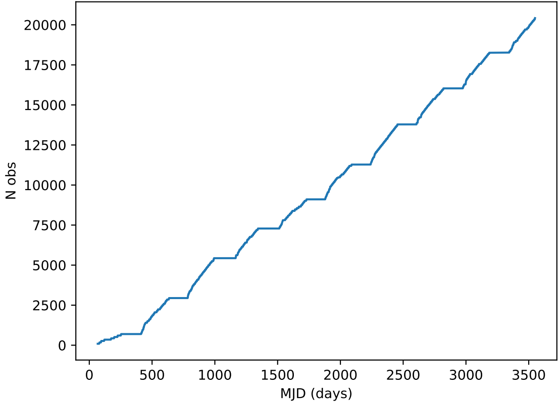
too_elab_heavy_r128_d3_gz_v3.4_10yrs all bands: DD:ELAISS1 Cumulative NVisits
