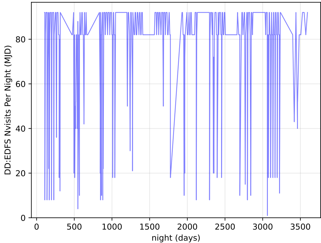
too_elab_heavy_r128_d3_gz_v3.4_10yrs all bands: DD:EDFS Nvisits Per Night
