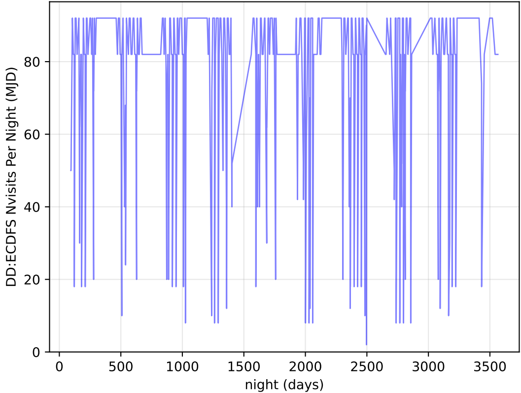
too_elab_heavy_r128_d3_gz_v3.4_10yrs all bands: DD:ECDFS Nvisits Per Night
