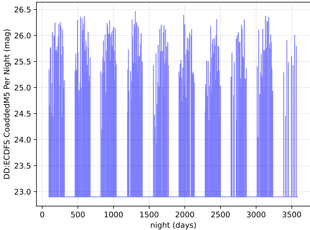
too_elab_heavy_r128_d3_gz_v3.4_10yrs r band: DD:ECDFS CoaddedM5 Per Night
