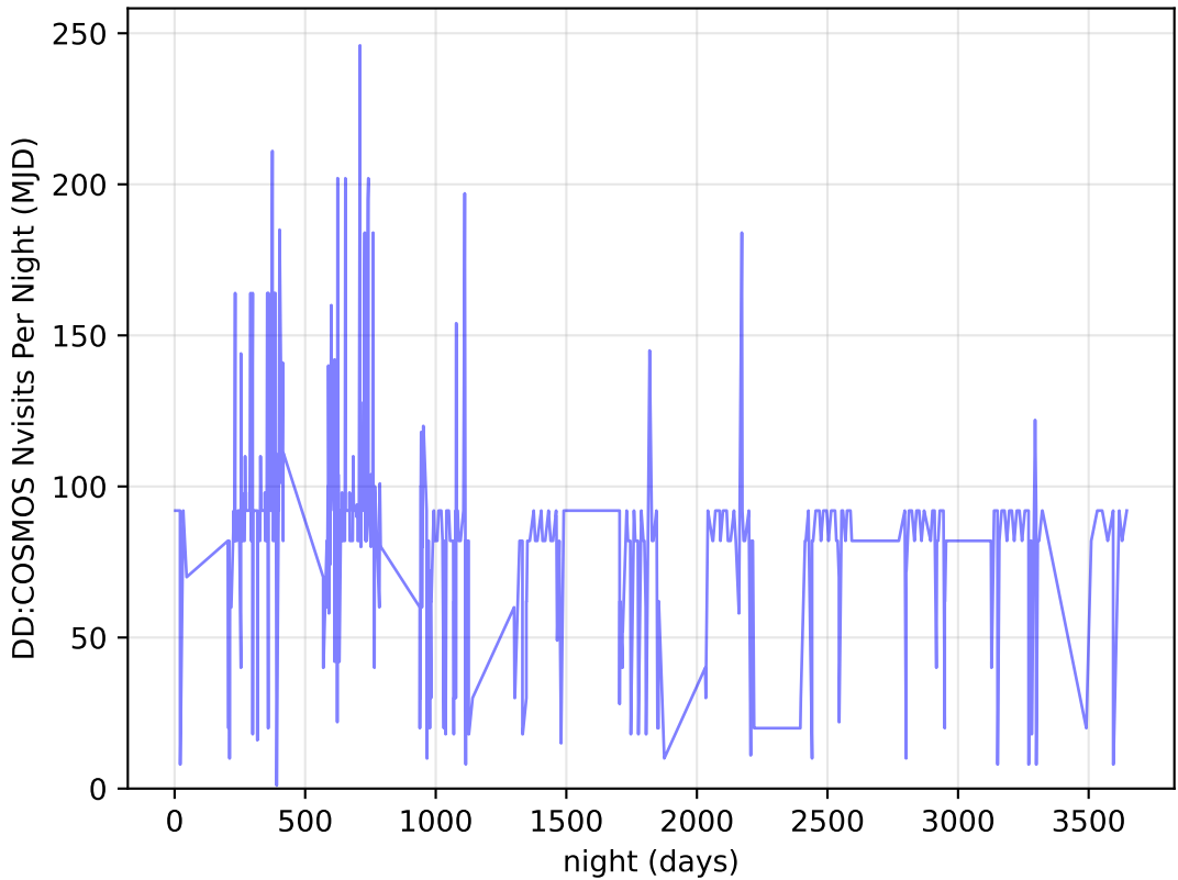
too_elab_heavy_r128_d3_gz_v3.4_10yrs all bands: DD:COSMOS Nvisits Per Night
