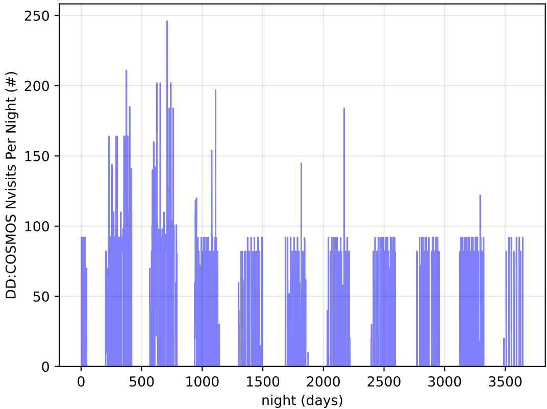
too_elab_heavy_r128_d3_gz_v3.4_10yrs all bands: DD: COSMOS Nvisits Per Night
