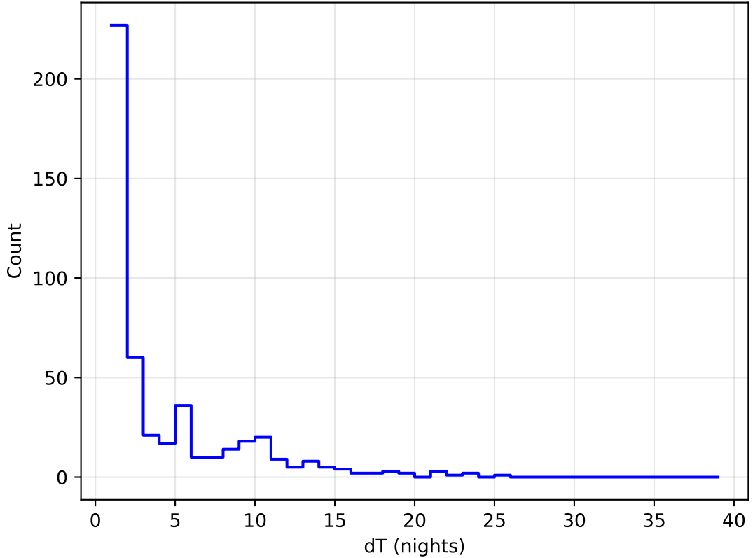
too_elab_heavy_r128_d3_gz_v3.4_10yrs all bands: DD: COSMOS Delta Nights Histogram
